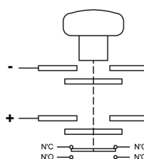
Connection Diagram
