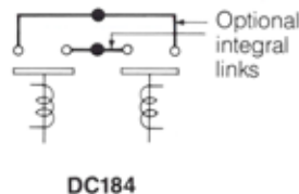
AUXILIARY CONTACTS
